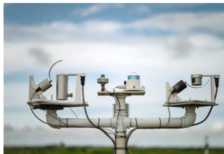
No.5 “TInstrument Suite with Multi-filter Rotating Shadow Band Radiometer, 23 June 2014” © Terri Weifenbach
